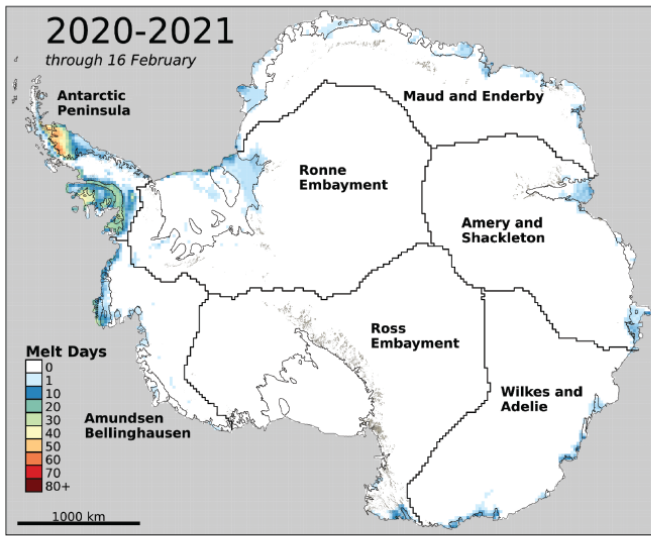
Antarctica Cumulative Melt Days, November 1, 2020 to February 16, 2021
