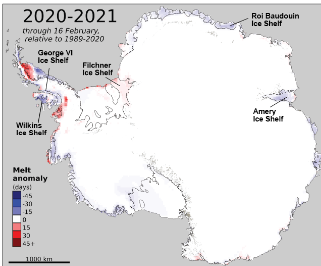
Antarctica Melt Days, Difference from Average November 1, 2020 to February 16, 2021
